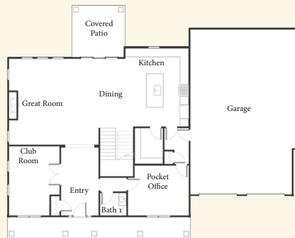
Alternate First Floor Plan
